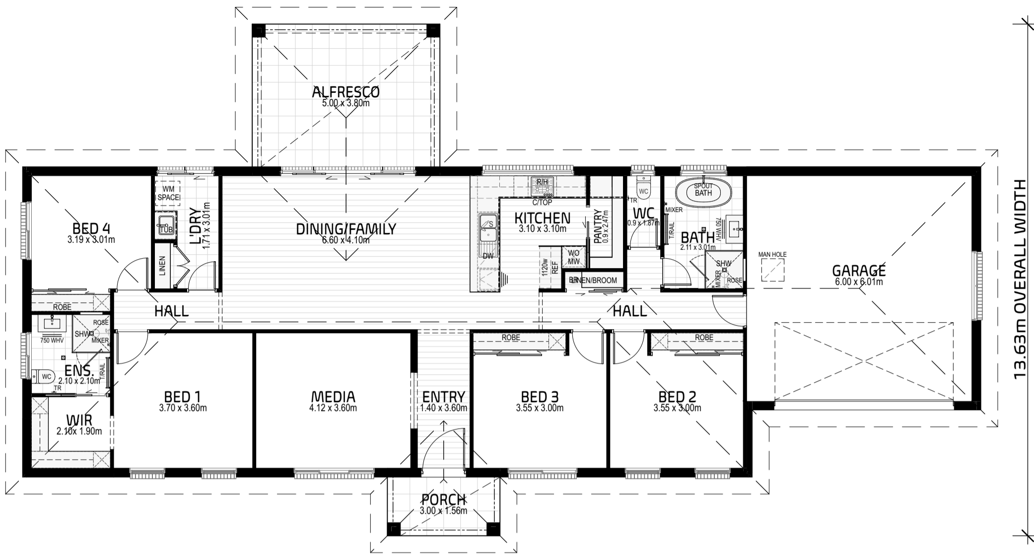
ROYAL 224 RHG FLOOR PLAN
