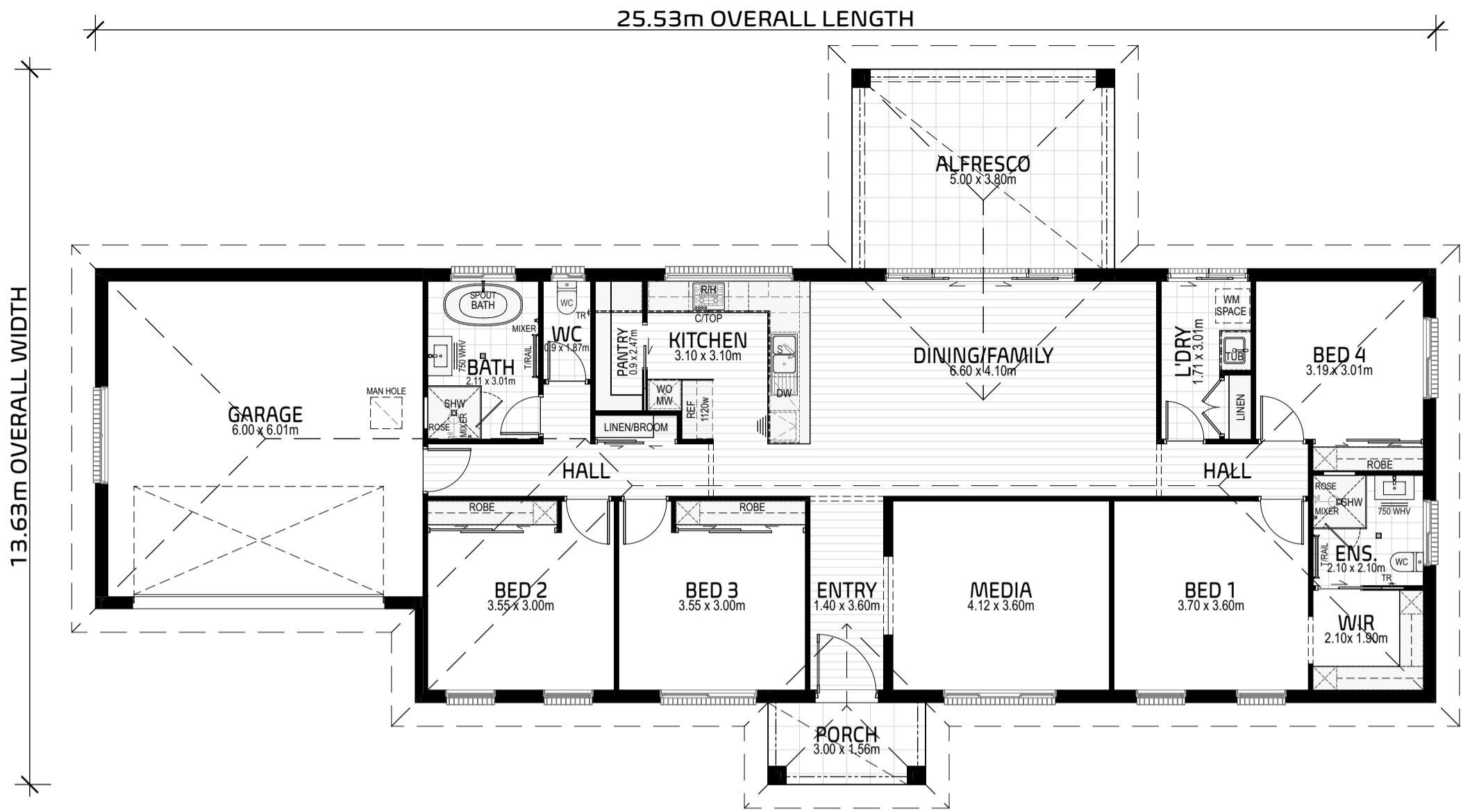
ROYAL 224 LHG FLOOR PLAN SCALE 1:100
